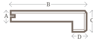
3/4" Euro Nosing
